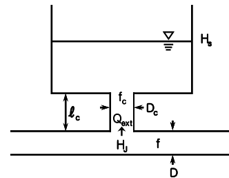
Fig. 1. A schematic for a surge tank.
